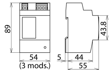
Dimension drawing PSU DC24 30W
