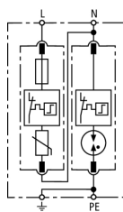
Basic circuit diagram DG M TT 2P CI 275
