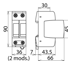
Dimension drawing DG M TT 2P CI 275
