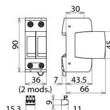
Dimension drawing DG M TN CI 275
