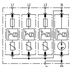
Basic circuit diagram DG M TT CI 275
