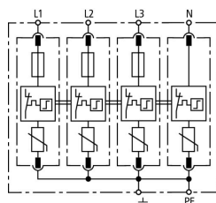
Basic circuit diagram DG M TNS CI 275
