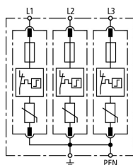
Basic circuit diagram DG M TNC CI 275
