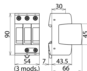
Dimension drawing DG M TNC CI 275
