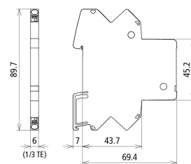
Dimension drawing BCO CL2 B 180
