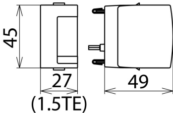
Dimension drawing DG MOD E DC 900
