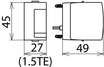
Dimension drawing DG MOD E DC 550
