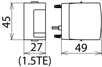
Dimension drawing DG MOD E DC 242
