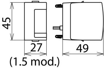
Dimension drawing DG MOD E DC 60
