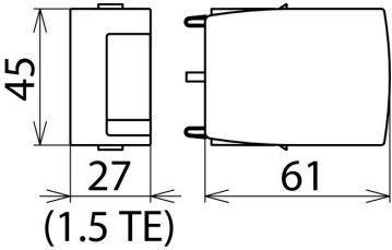
Dimension drawing DG MOD E H LI 1000
