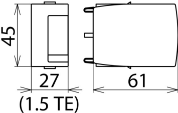
Dimension drawing DG MOD E H LI 1000
