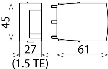
Dimension drawing DG MOD E H LI 275
