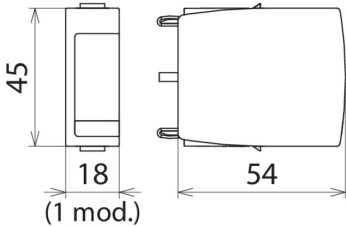
Dimension drawing DG MOD H A NPE
