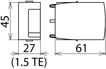
Dimension drawing DG MOD E CI 440
