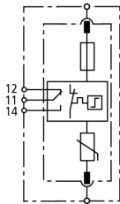
Basic circuit diagramDG MOD E CI 440
