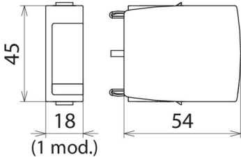
Dimension drawing DG MOD A NPE
