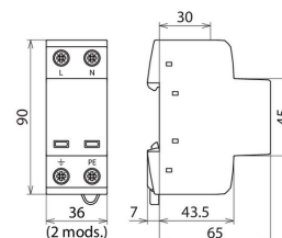
Dimension drawing DSH TN 255
