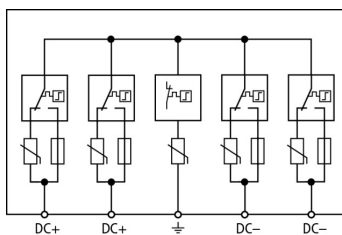
Basic circuit diagram DCU YPV SCI 1000 2M
