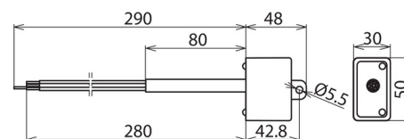
Dimension drawing DCOR L 2P 275 SO IP
