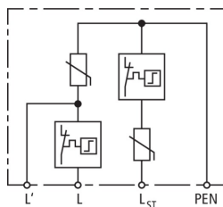
Basic circuit diagram DCOR L 2P 275 SO LT
