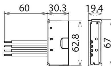
Dimension drawing DCOR L 2P 275 SO LT
