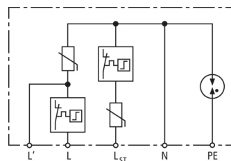
Basic circuit diagram DEHNcord
