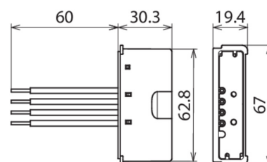
Dimension drawing DCOR L 2P SN1864
