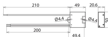
Dimension drawing DCOR L 2P 320
