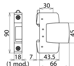
Dimension drawing DK 25
