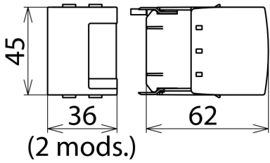
Dimension drawing DV MOD NPE 100
