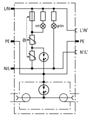
Basic circuit diagram DPRO 230 TV
