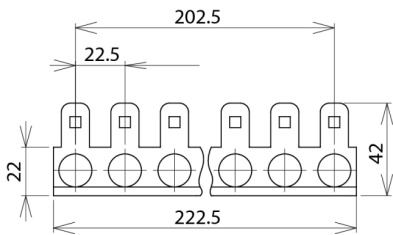
Dimension drawing MB2 10 LSA
