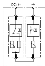
Basic circuit diagram DG S PV SCI 150
