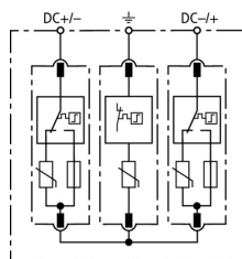
Basic circuit diagram DG M YPV SCI 1200
