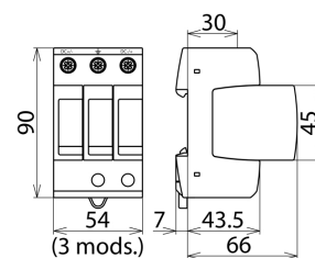
Dimension drawing DG M YPV SCI 1200
