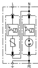
Basic circuit diagram DG M TT 2P 385
