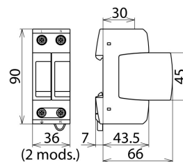
Dimension drawing DG M TT 2P 385
