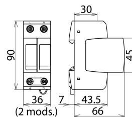
Dimension drawing DG M TT 2P 320
