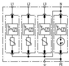
Basic circuit diagram DG M TT 385
