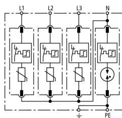
Basic circuit diagram DG M TT 320
