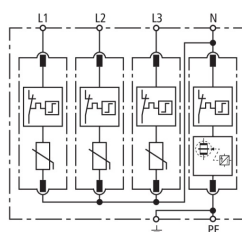
Basic circuit diagram DG M H TT 275
