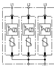
Basic circuit diagram DG M TNC 440
