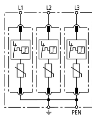
Basic circuit diagram DG M TNC 150
