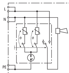
Basic circuit diagram DFL D 255
