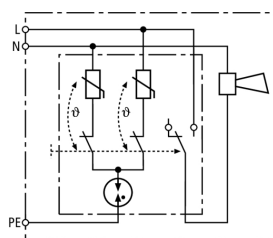
Basic circuit diagram DFL A 255
