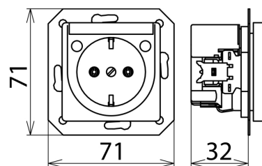
Dimension drawing NSM PRO TW
