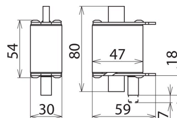
Dimension drawing V NH00 280 FM
