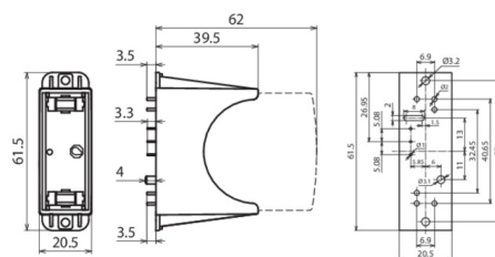
Dimension drawing DG PCB PV I 500 FM
