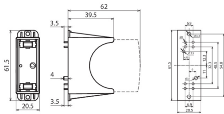
Dimension drawing DG PCB 275
