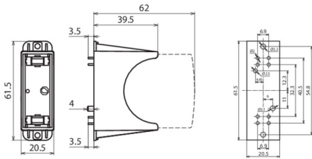
Dimension drawing DG PCB PV 500
