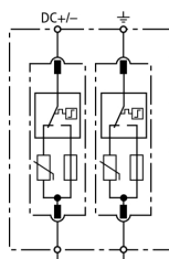
Basic circuit diagram DG SE PV SCI 1500
