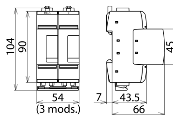
Dimension drawing DG SE PV SCI 1500
