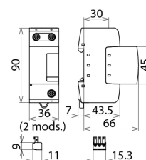
Dimension drawing DGPH M 255
